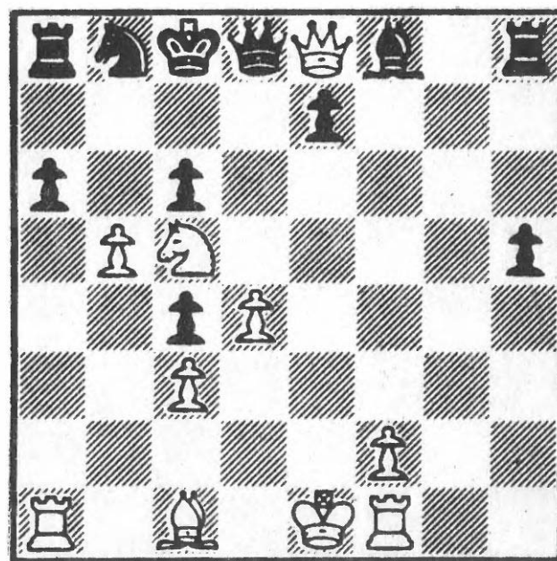
178 After 21...Qd8
